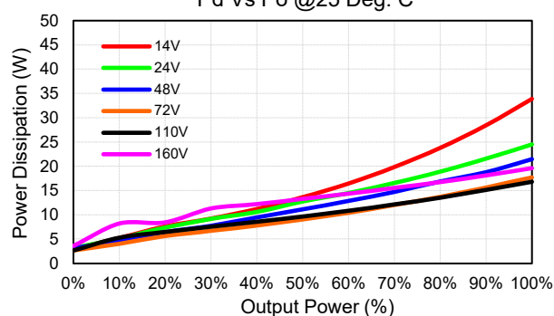
CFDH12R200-72S24 Pd Vs Po @25 Deg. C
