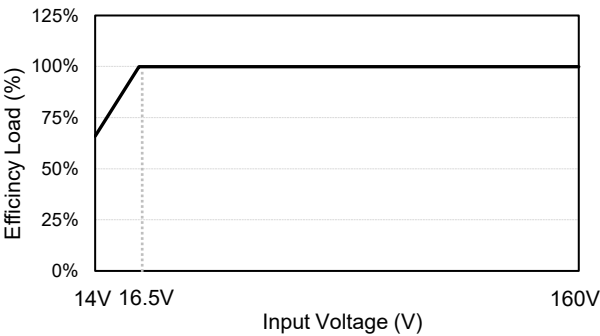
Typical Derating Curve VS Input Voltage
