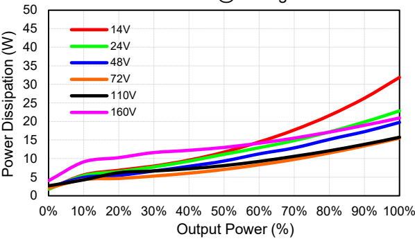
CFDH12R200-72S12 Pd Vs Po @25 Deg. C
