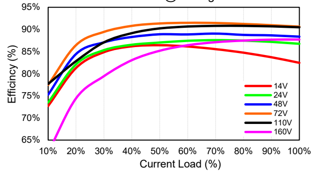
CFDH12R200-72S12 Eff Vs Io @25 Deg. C
