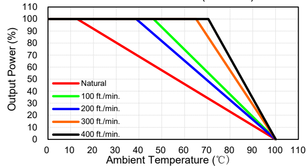
CFDH12R200-72S Derating Curve with Heatsink HBT127 (Vin=72V)
