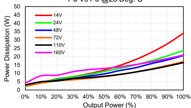
CFDH12R200-72S15 Pd Vs Po @25 Deg. C
