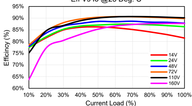
CFDH12R200-72S15 Eff Vs Io @25 Deg. C
