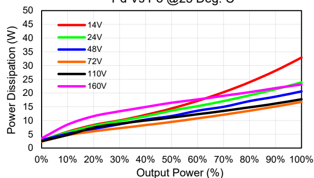
CFDH12R200-72S48 Pd Vs Po @25 Deg. C
