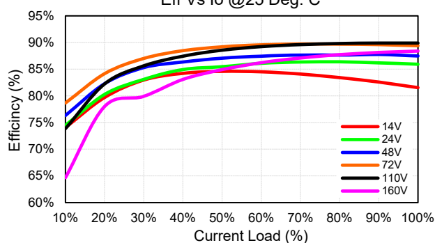
CFDH12R200-72S24 Eff Vs Io @25 Deg. C
