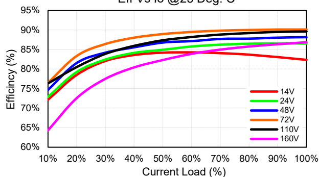
CFDH12R200-72S48 Eff Vs Io @25 Deg. C
